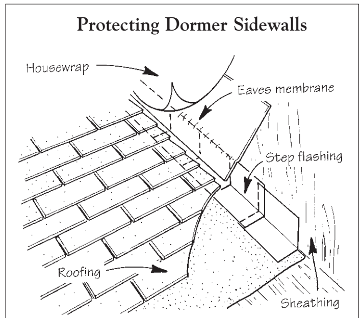
Figure 2. To protect dormer sidewalls, make sure the step flashings are installed behind the housewrap. At areas where water accumulates, the author lifts the housewrap and adds a strip of self-adhering eaves membrane over the step flashing.
